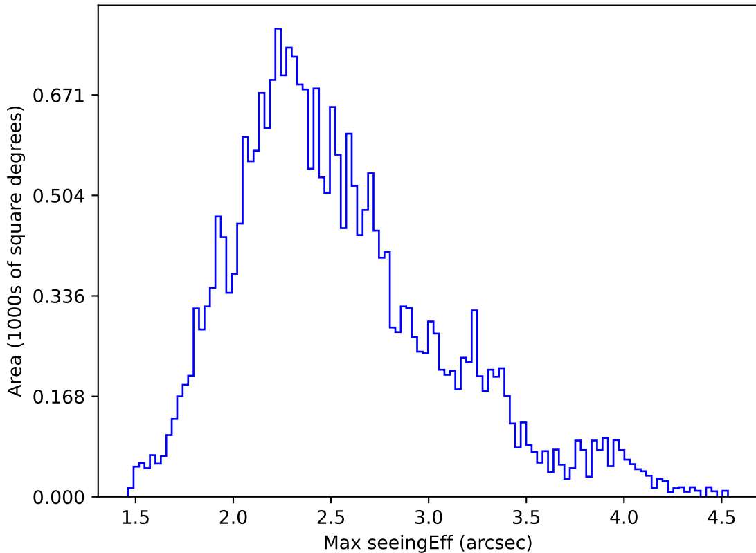
noroll_mjdp60_v3.4_10yrs All sky r band: Max seeingEff
