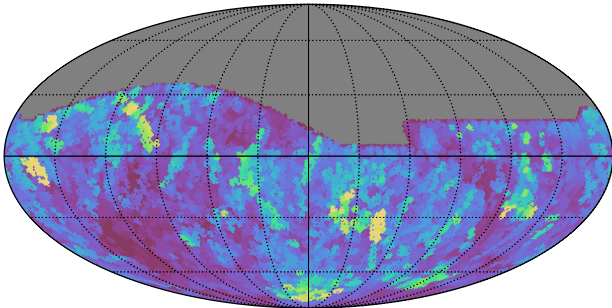
noroll_mjdp60_v3.4_10yrs All sky i band: Max seeingEff
