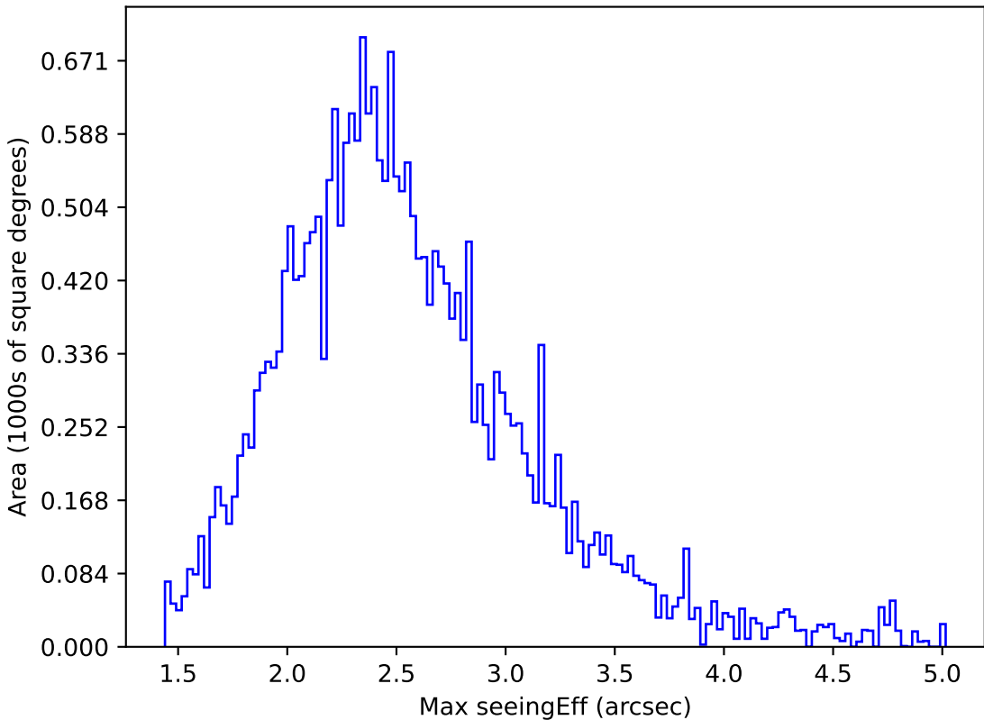
noroll_mjdp60_v3.4_10yrs All sky i band: Max seeingEff
