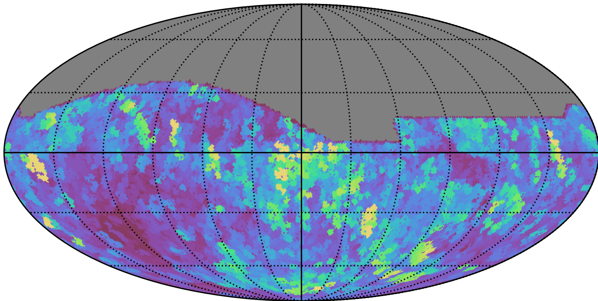
noroll_mjdp60_v3.4_10yrs All sky all bands: Max seeingEff
