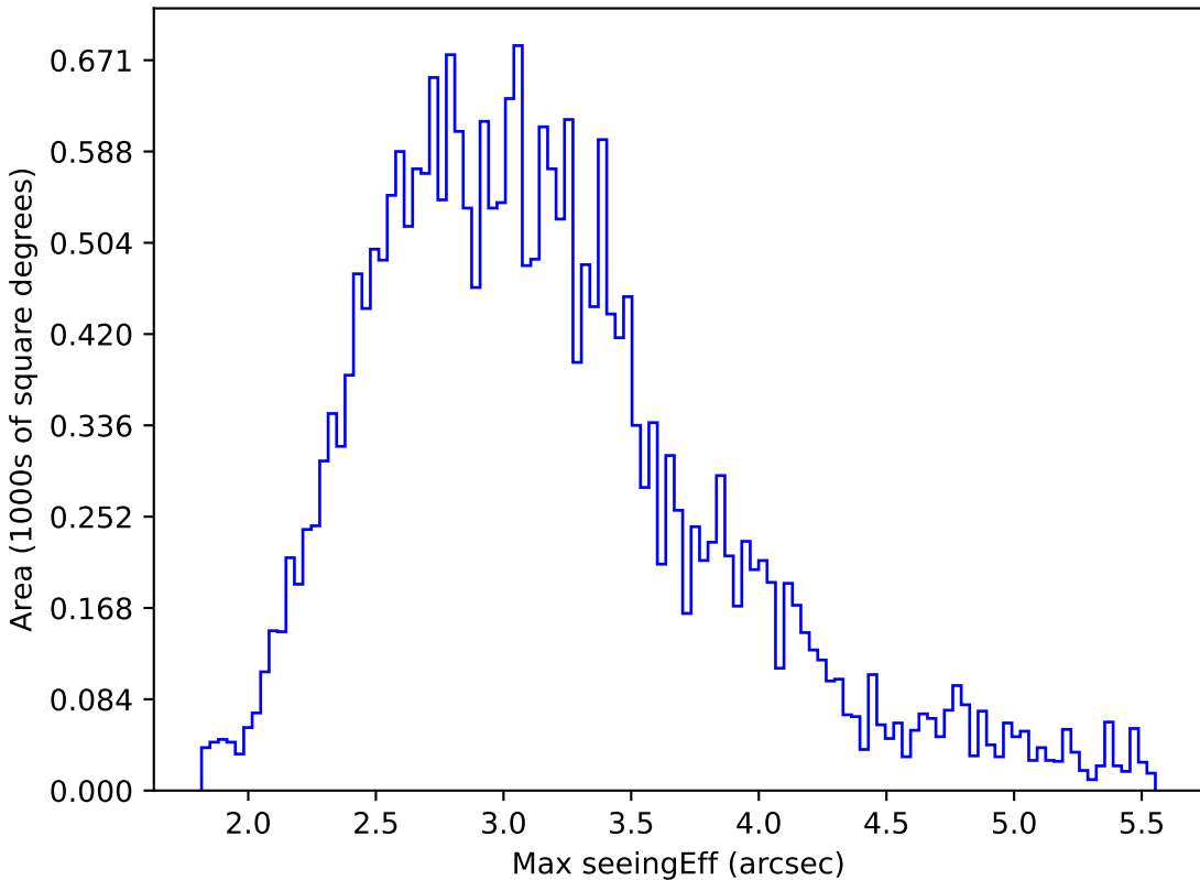
noroll_mjdp60_v3.4_10yrs All sky all bands: Max seeingEff
