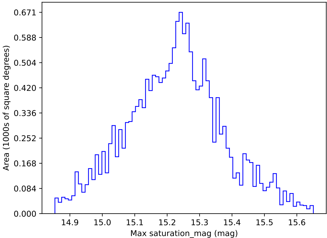
noroll_mjdp60_v3.4_10yrs WFD z band: Max saturation_mag
