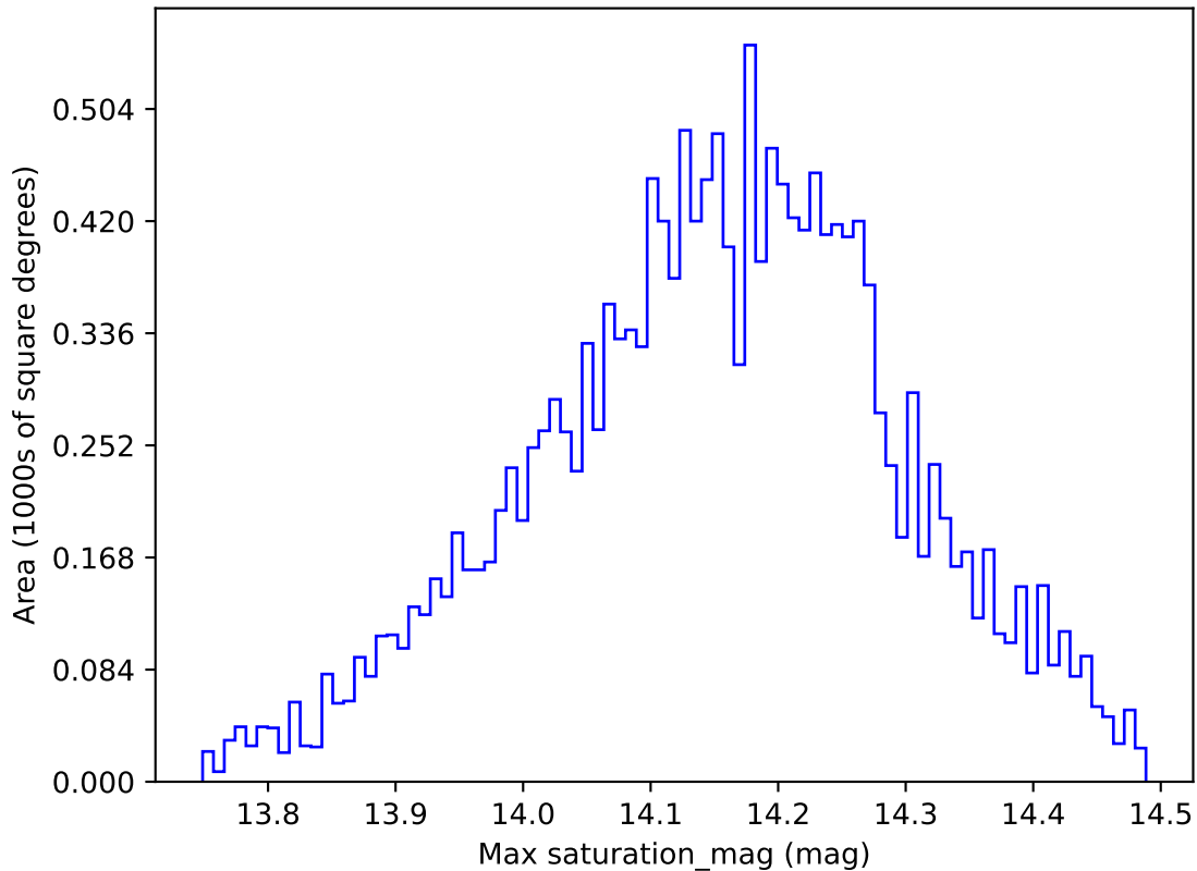
noroll_mjdp60_v3.4_10yrs WFD y band: Max saturation_mag
