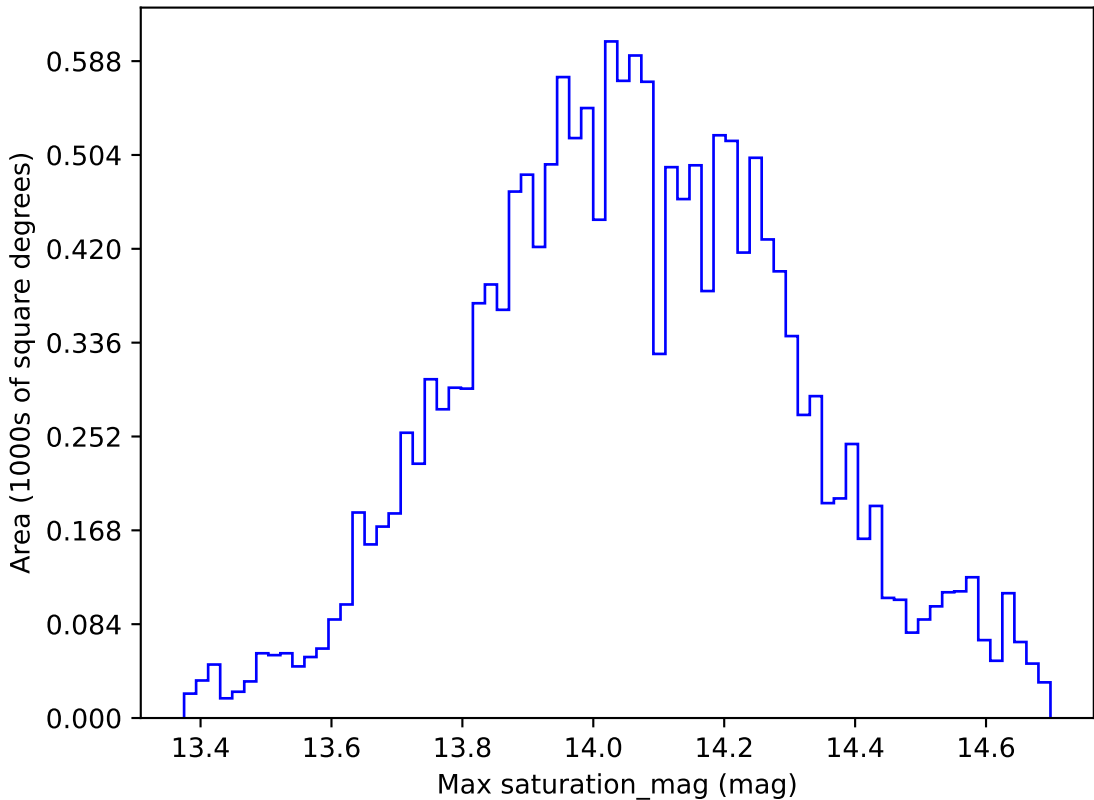
noroll_mjdp60_v3.4_10yrs WFD u band: Max saturation_mag
