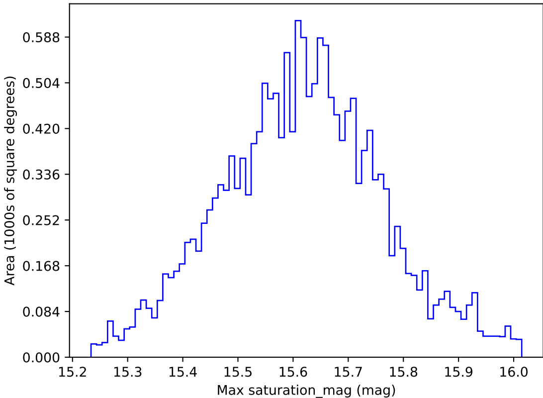
noroll_mjdp60_v3.4_10yrs WFD i band: Max saturation_mag
