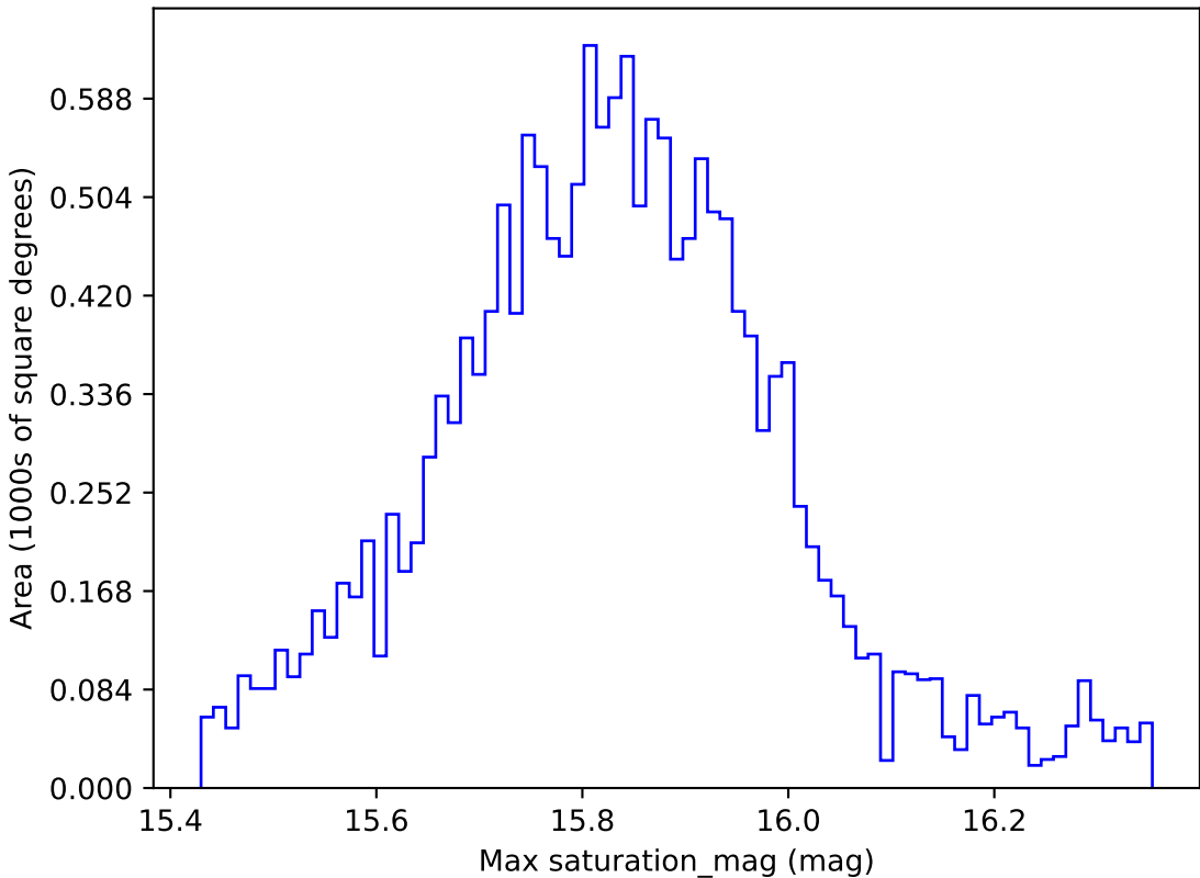
noroll_mjdp60_v3.4_10yrs WFD all bands: Max saturation_mag
