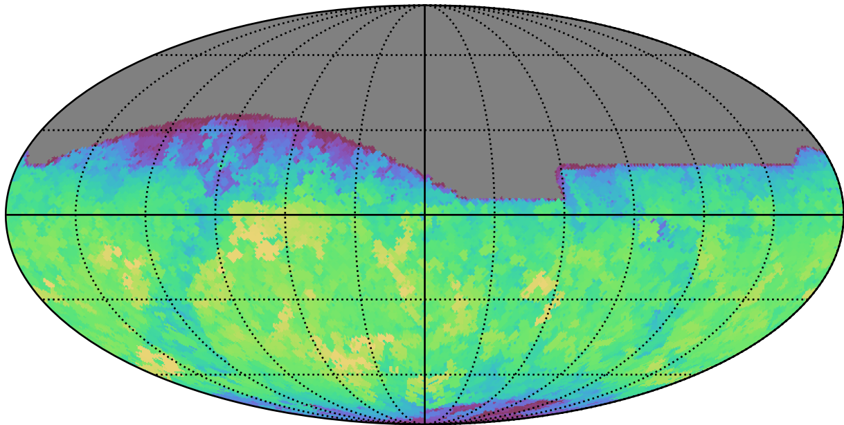
noroll_mjdp60_v3.4_10yrs All sky z band: Max saturation_mag
