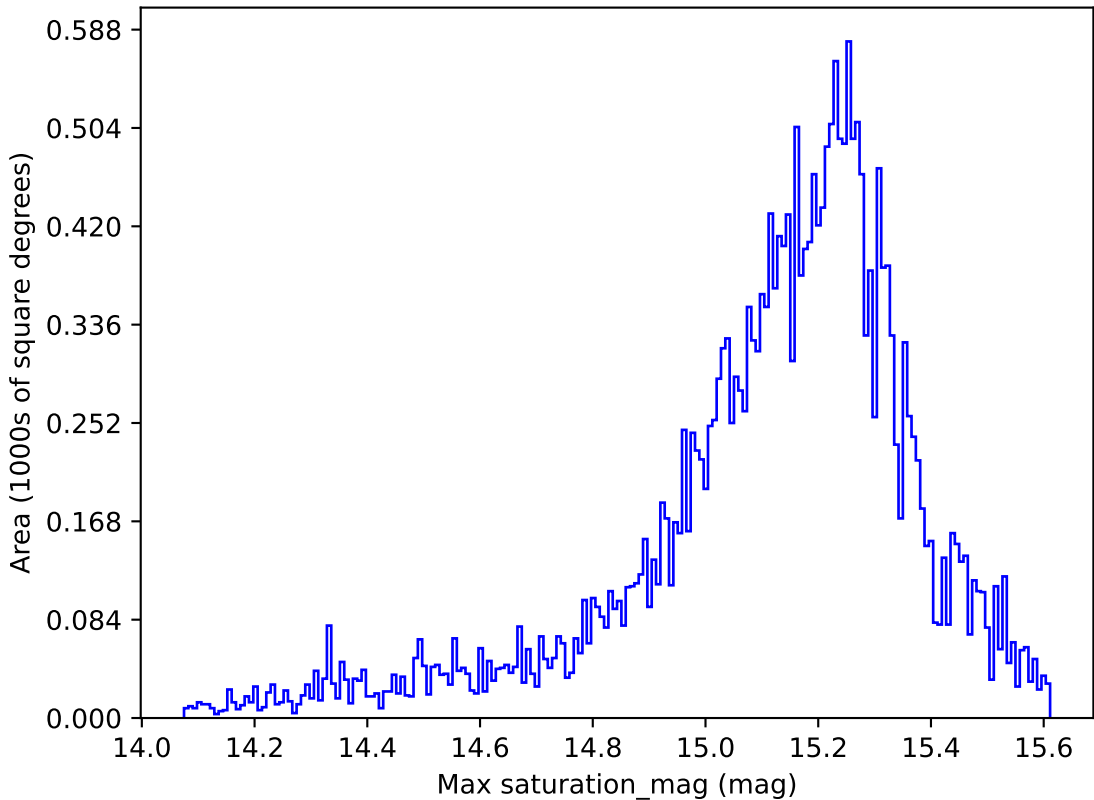
noroll_mjdp60_v3.4_10yrs All sky z band: Max saturation_mag
