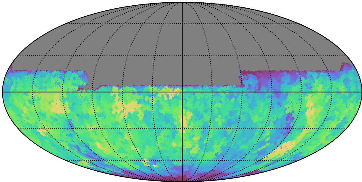
noroll_mjdp60_v3.4_10yrs All sky u band: Max saturation_mag
