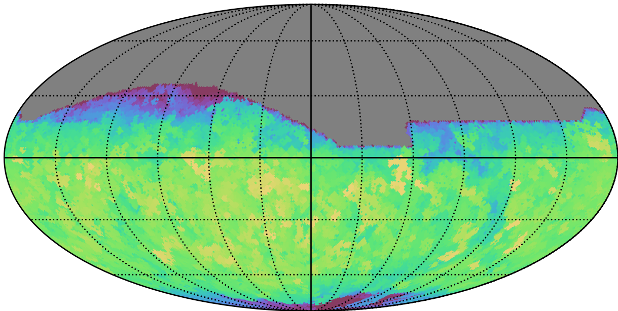
noroll_mjdp60_v3.4_10yrs All sky r band: Max saturation_mag
