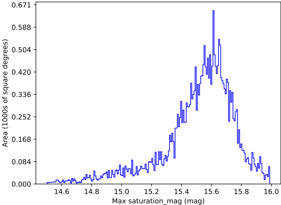
noroll_mjdp60_v3.4_10yrs All sky i band: Max saturation_mag
