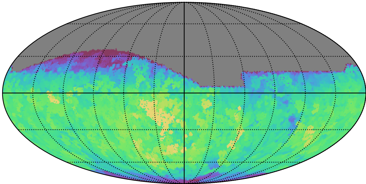
noroll_mjdp60_v3.4_10yrs All sky g band: Max saturation_mag
