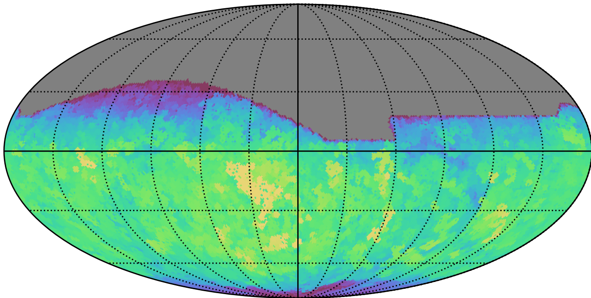
noroll_mjdp60_v3.4_10yrs All sky all bands: Max saturation_mag
