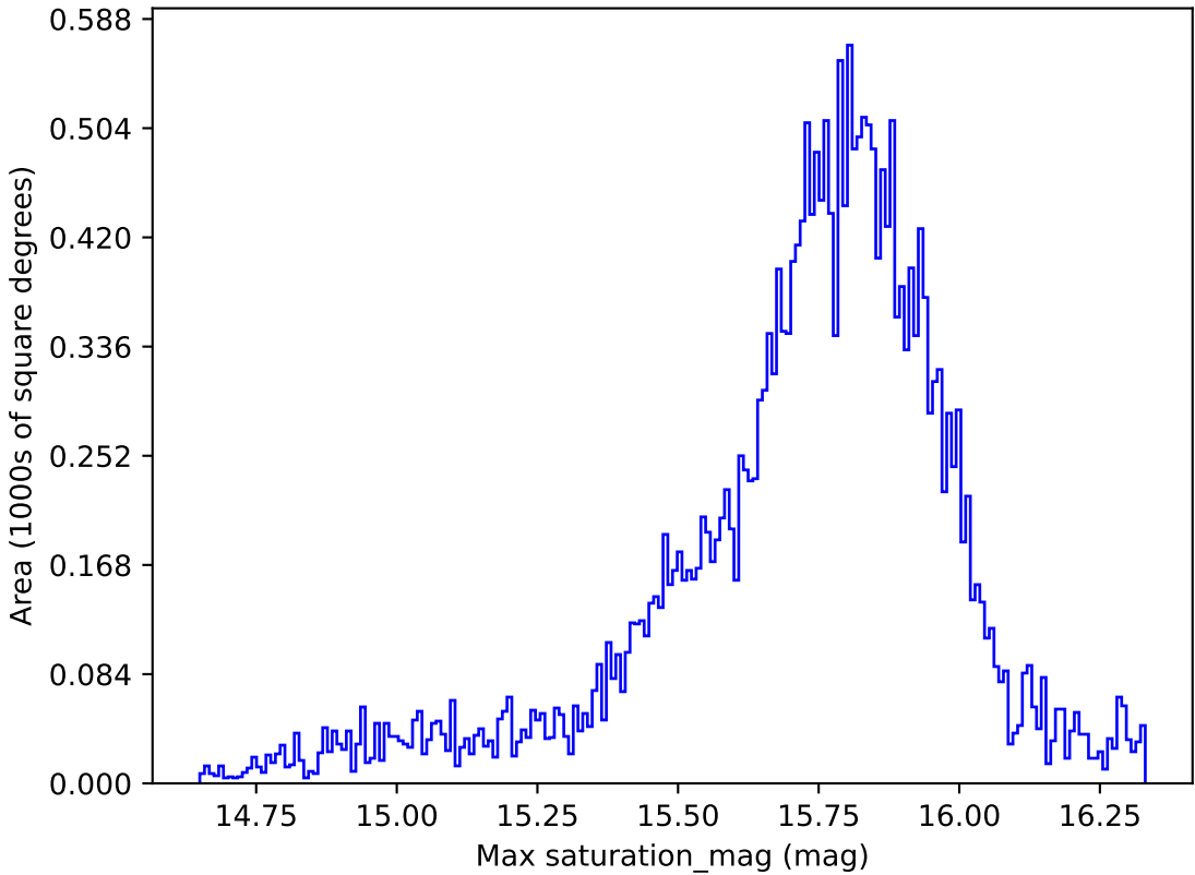
noroll_mjdp60_v3.4_10yrs All sky all bands: Max saturation_mag
