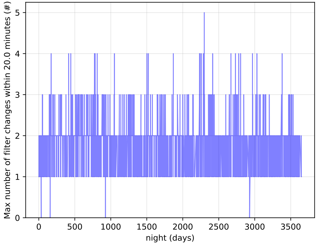
noroll_mjdp60_v3.4_10yrs Per Night: Max number of filter changes within 20.0 minutes
