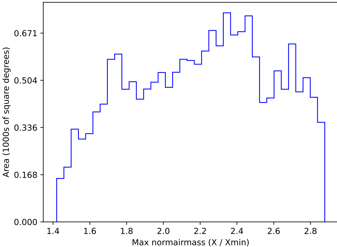
noroll_mjdp60_v3.4_10yrs WFD z band: Max normairmass
