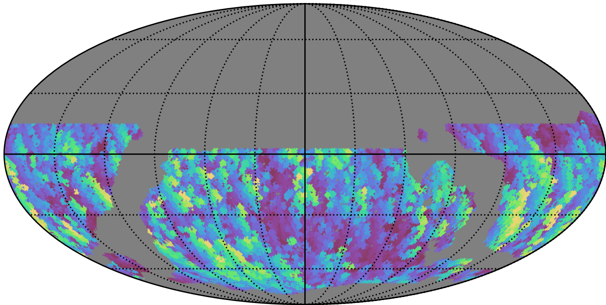
noroll_mjdp60_v3.4_10yrs WFD y band: Max normairmass
