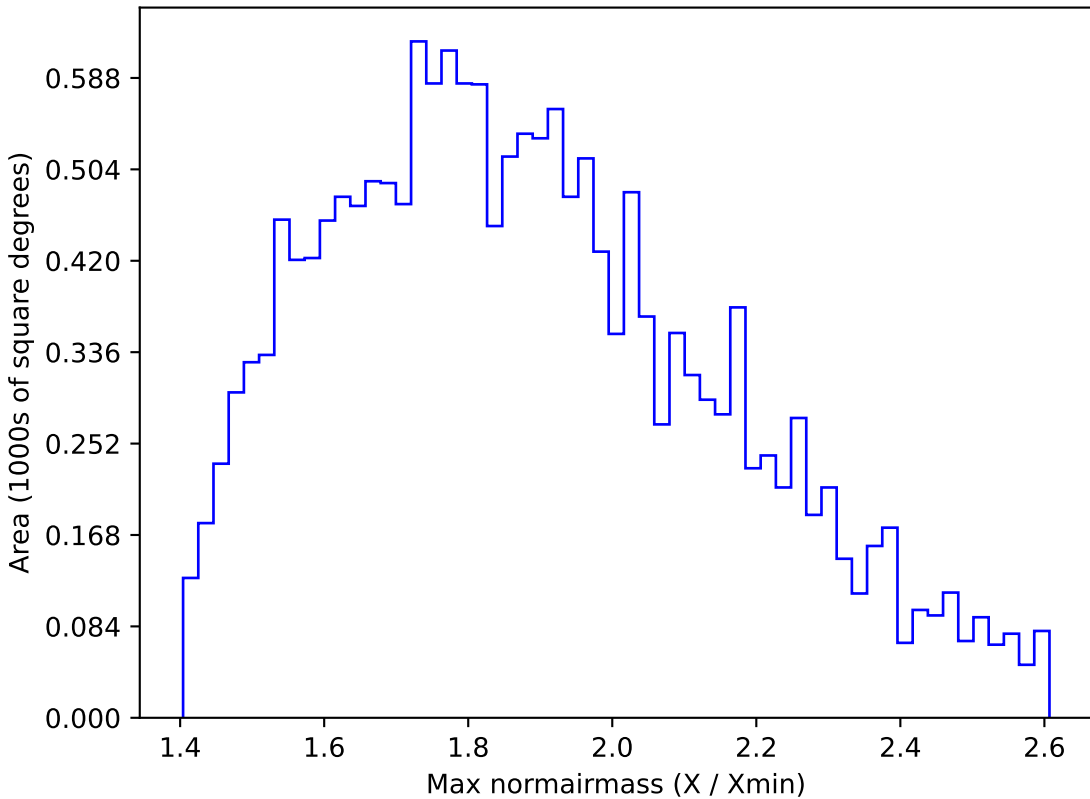
noroll_mjdp60_v3.4_10yrs WFD y band: Max normairmass
