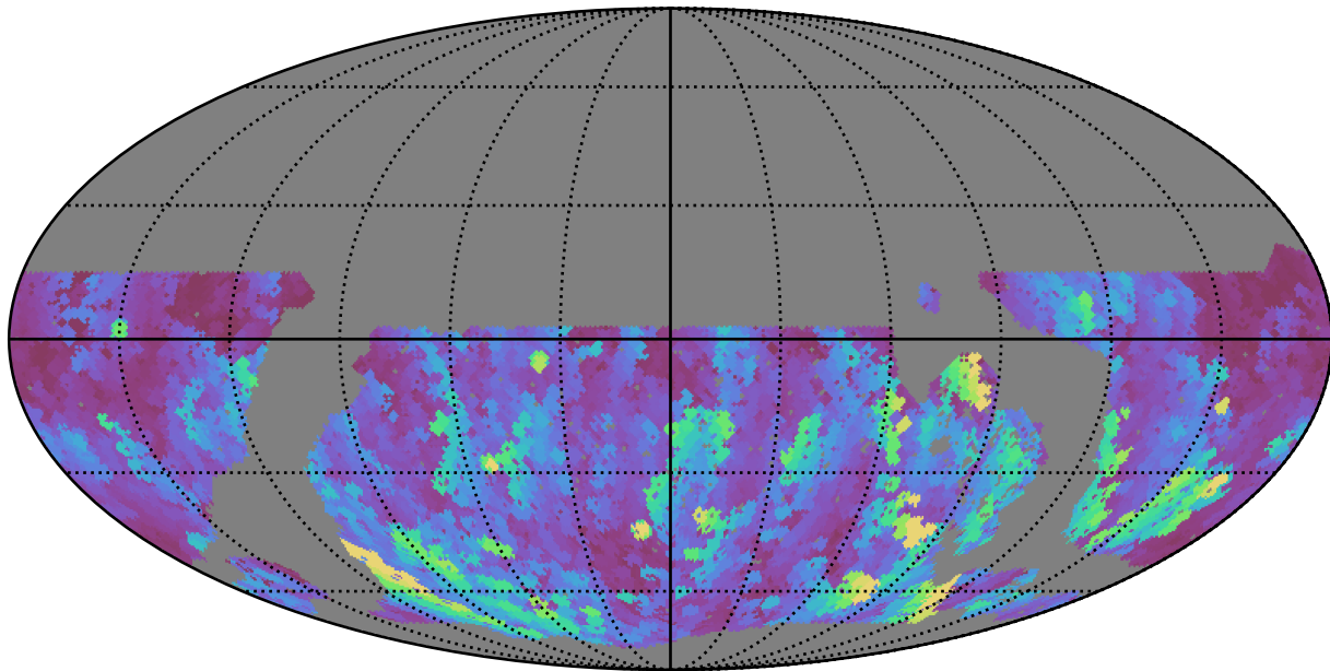
noroll_mjdp60_v3.4_10yrs WFD u band: Max normairmass
