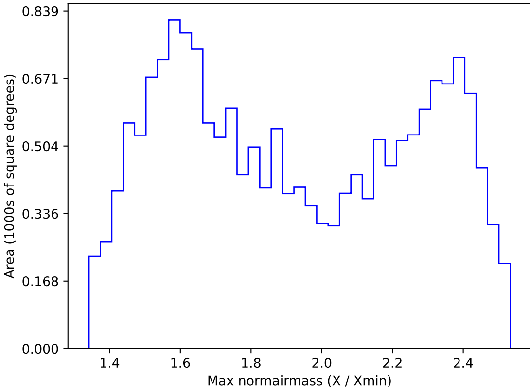
noroll_mjdp60_v3.4_10yrs WFD r band: Max normairmass
