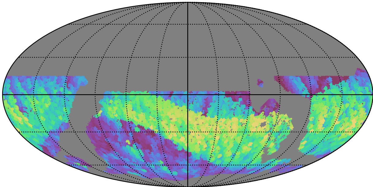
noroll_mjdp60_v3.4_10yrs WFD i band: Max normairmass
