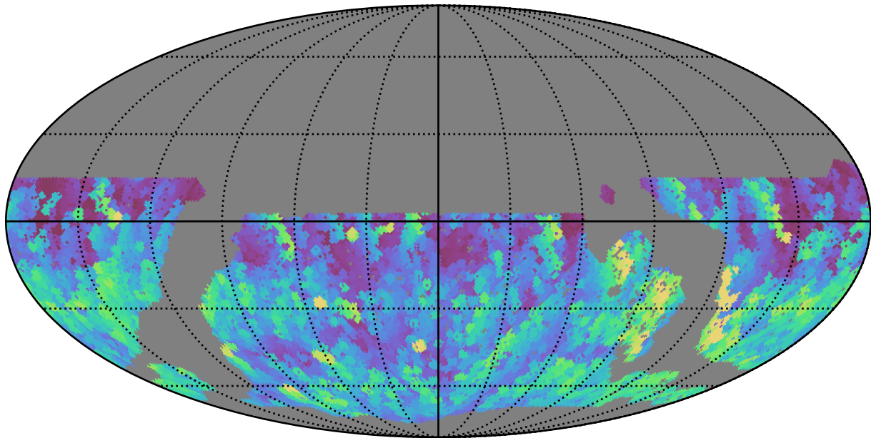
noroll_mjdp60_v3.4_10yrs WFD g band: Max normairmass
