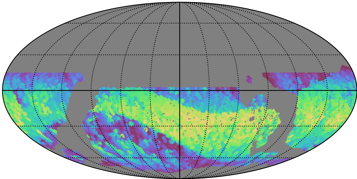
noroll_mjdp60_v3.4_10yrs WFD all bands: Max normairmass
