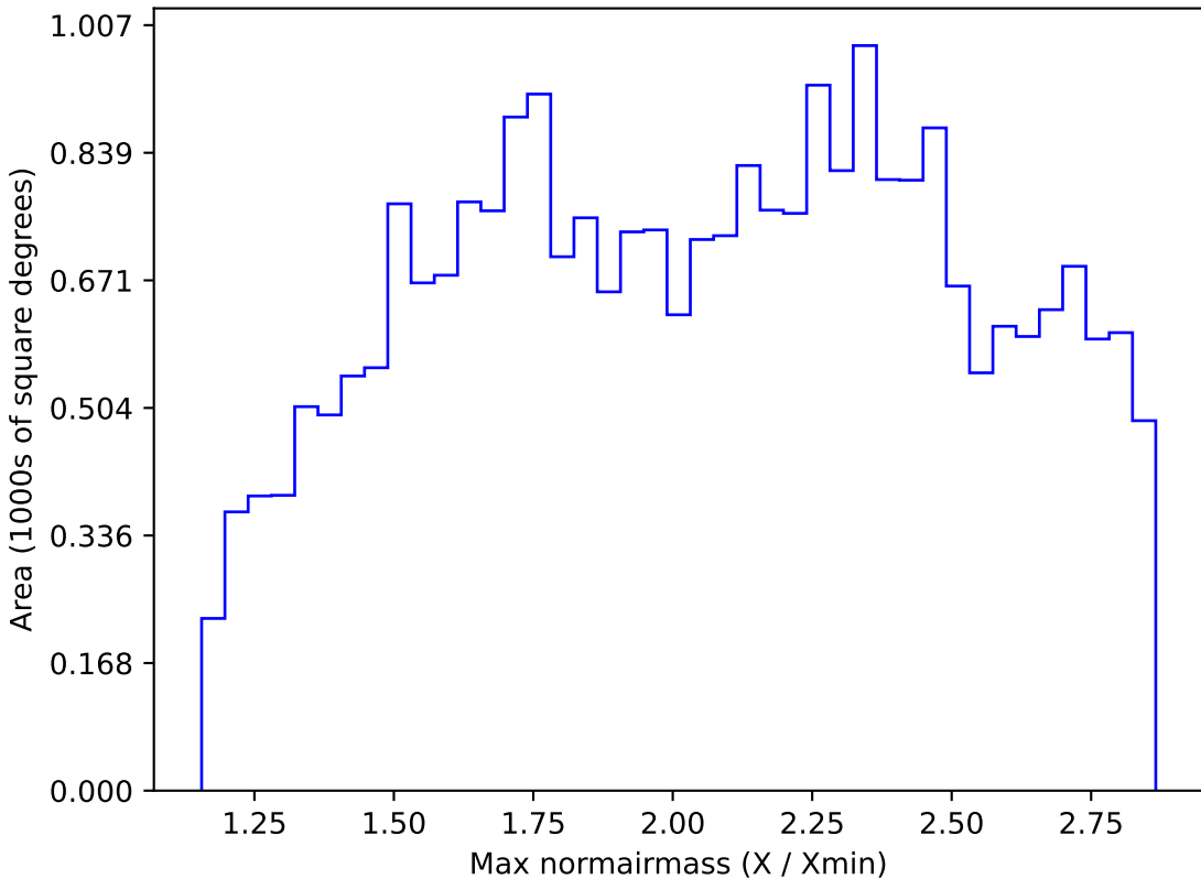
noroll_mjdp60_v3.4_10yrs All sky z band: Max normairmass
