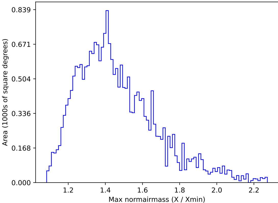
noroll_mjdp60_v3.4_10yrs All sky u band: Max normairmass
