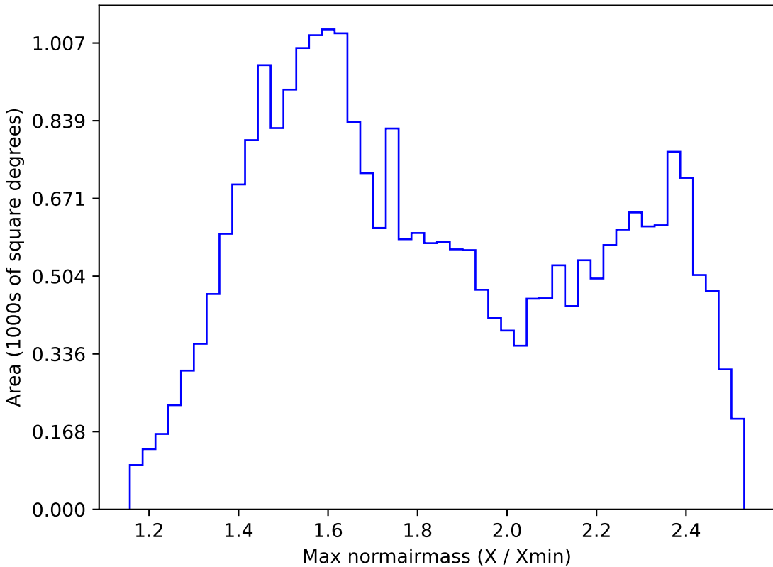
noroll_mjdp60_v3.4_10yrs All sky r band: Max normairmass
