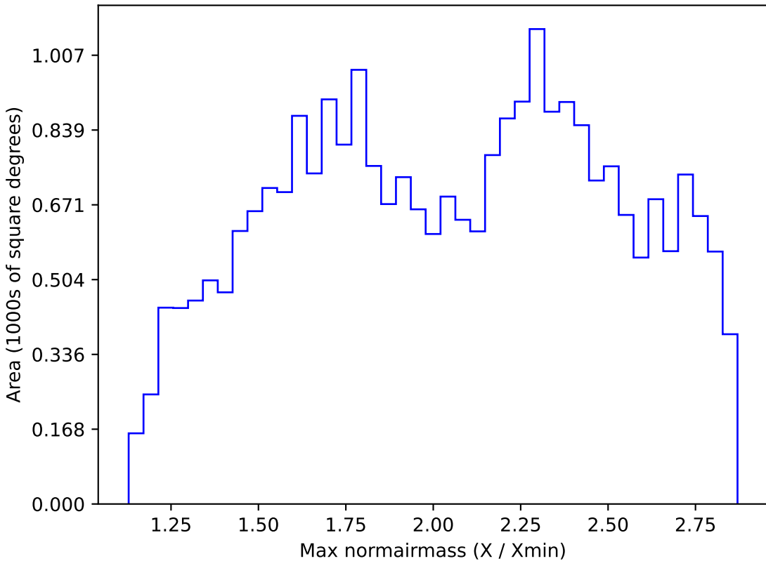
noroll_mjdp60_v3.4_10yrs All sky i band: Max normairmass
