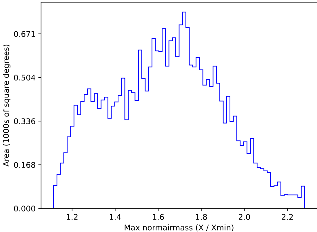
noroll_mjdp60_v3.4_10yrs All sky g band: Max normairmass
