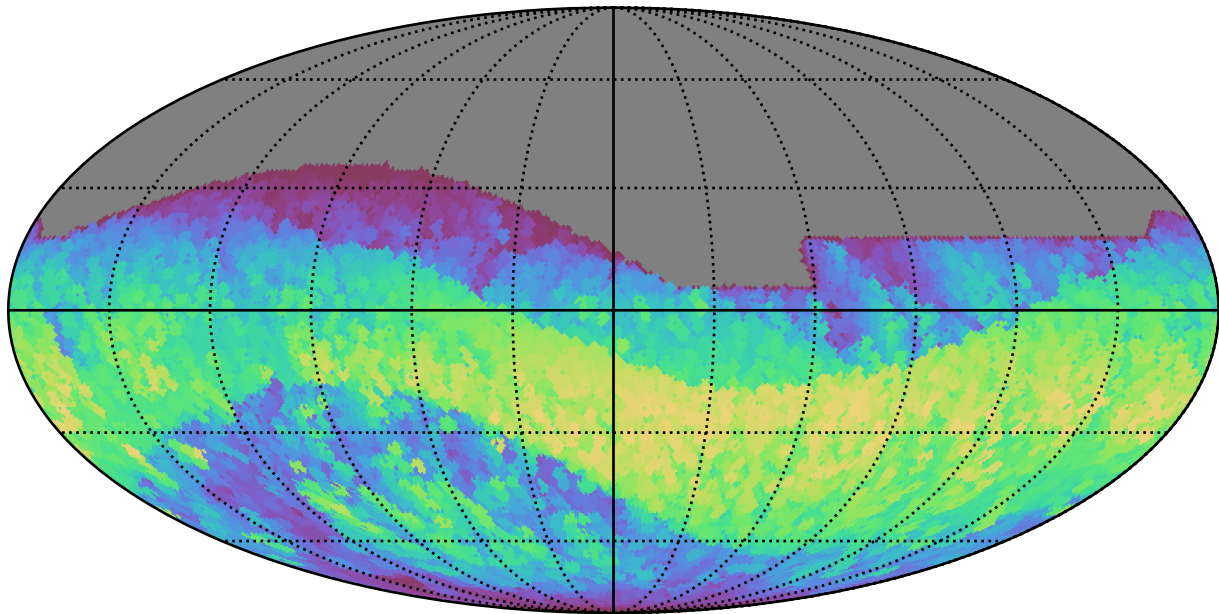
noroll_mjdp60_v3.4_10yrs All sky all bands: Max normairmass
