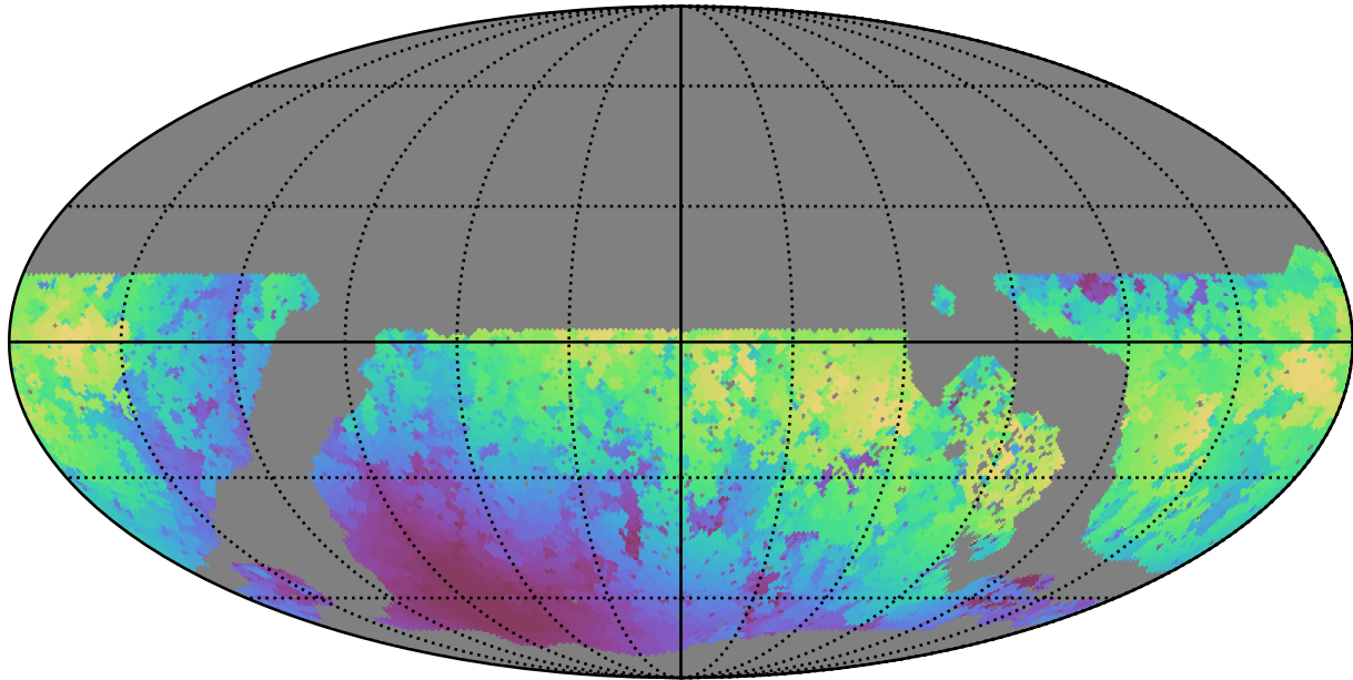
noroll_mjdp60_v3.4_10yrs WFD y band: Max moonDistance
