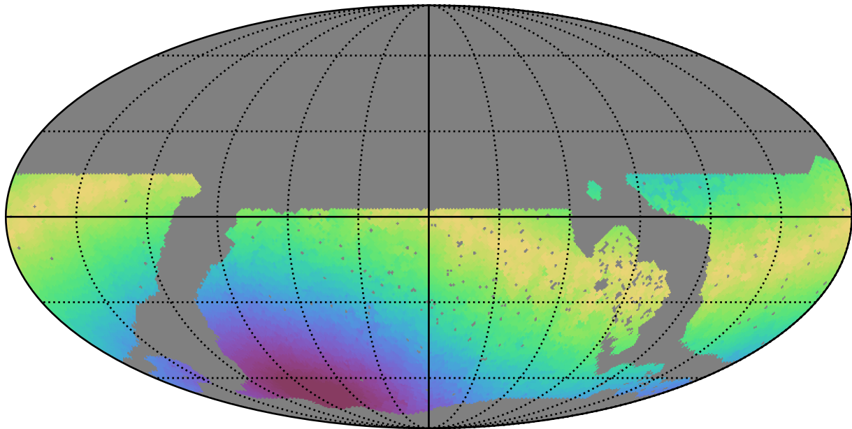
noroll_mjdp60_v3.4_10yrs WFD u band: Max moonDistance
