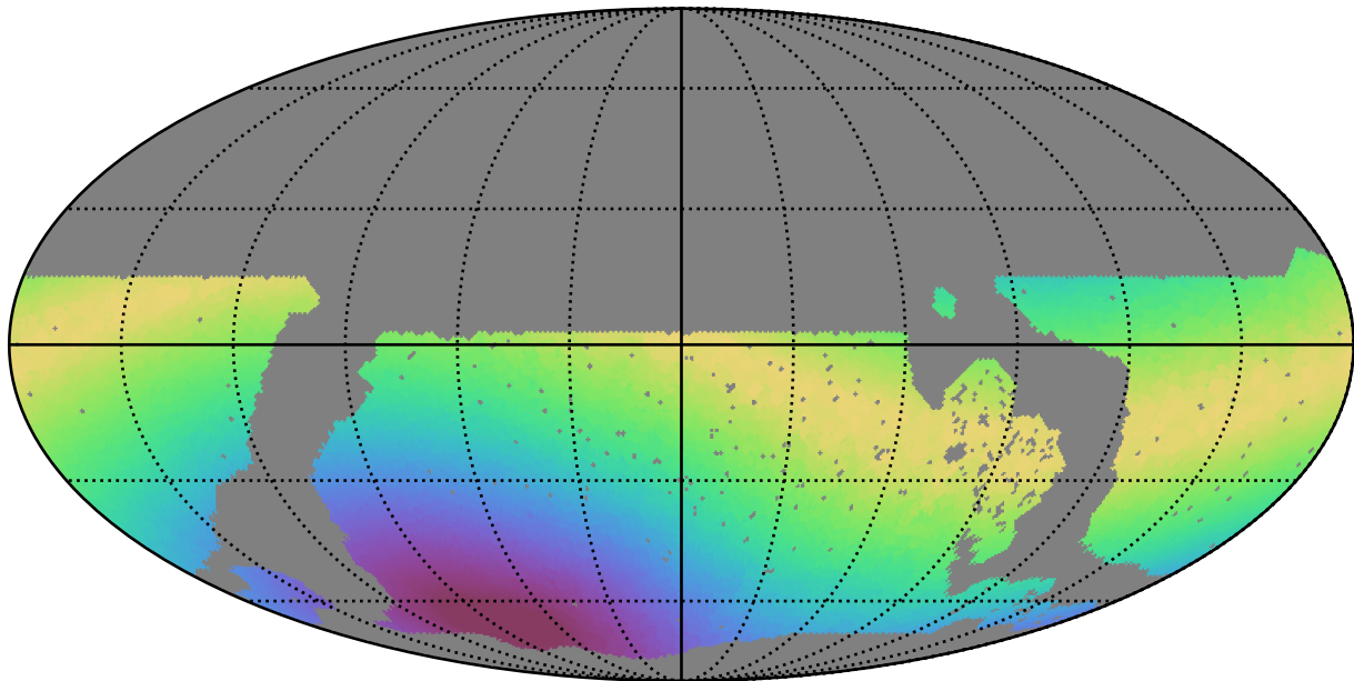
noroll_mjdp60_v3.4_10yrs WFD all bands: Max moonDistance
