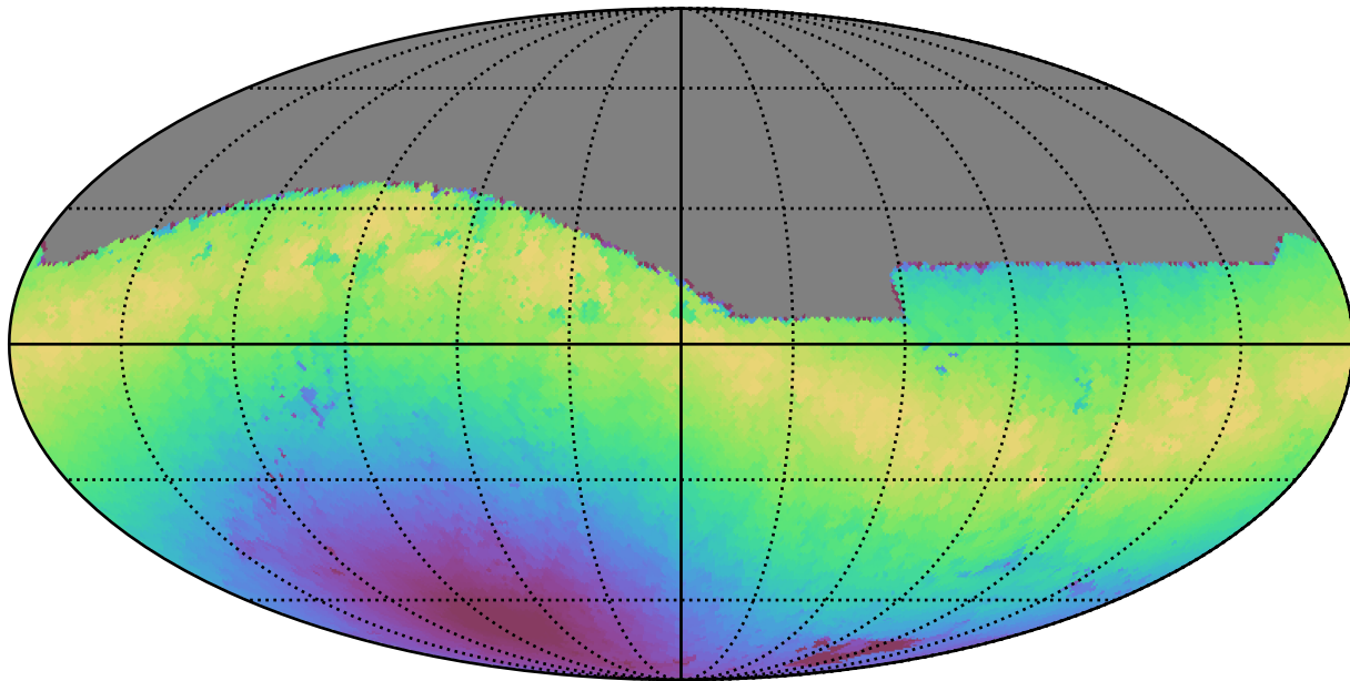
noroll_mjdp60_v3.4_10yrs All sky z band: Max moonDistance
