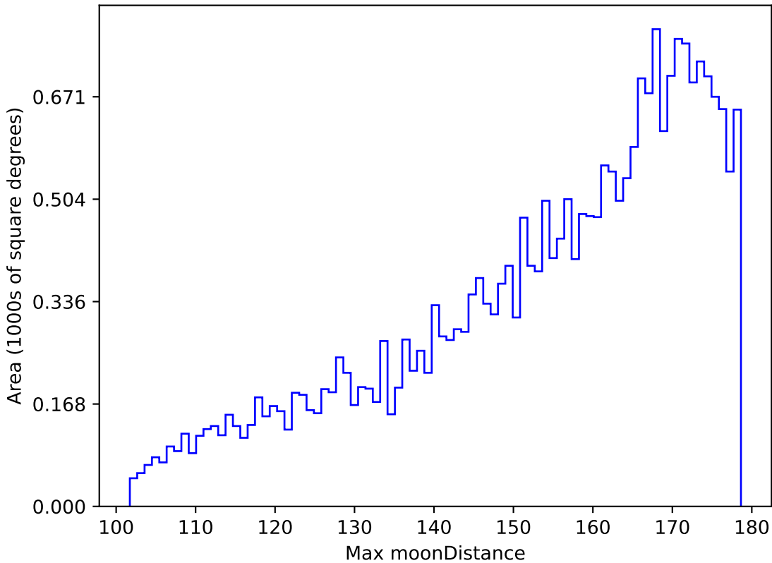
noroll_mjdp60_v3.4_10yrs All sky z band: Max moonDistance
