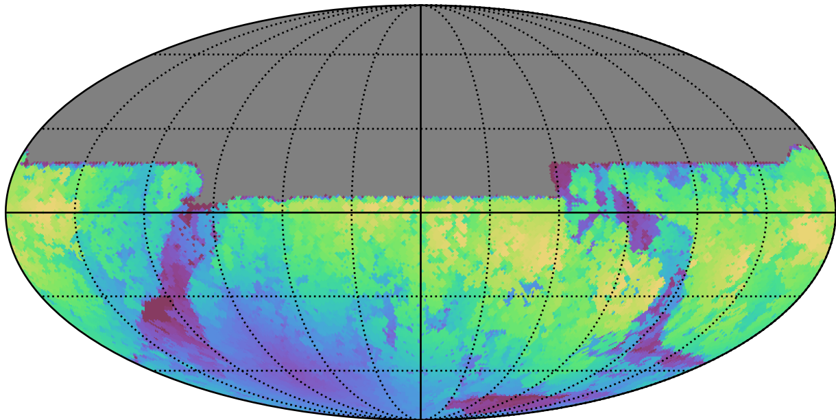
noroll_mjdp60_v3.4_10yrs All sky y band: Max moonDistance
