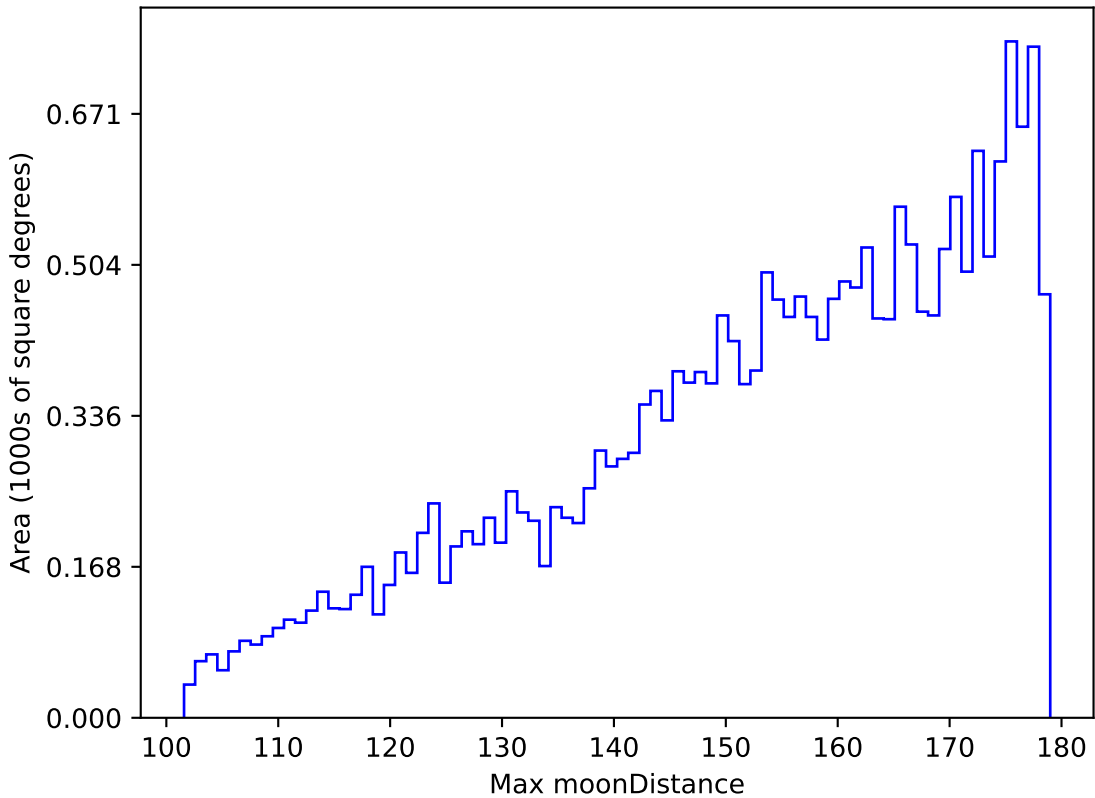
noroll_mjdp60_v3.4_10yrs All sky u band: Max moonDistance
