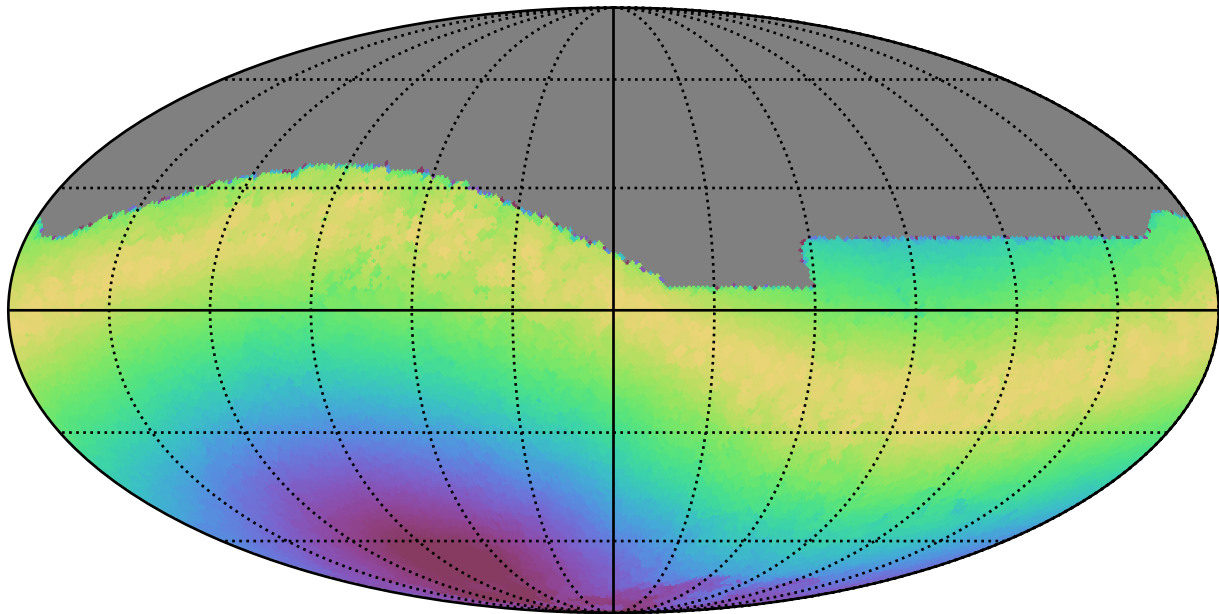
noroll_mjdp60_v3.4_10yrs All sky r band: Max moonDistance
