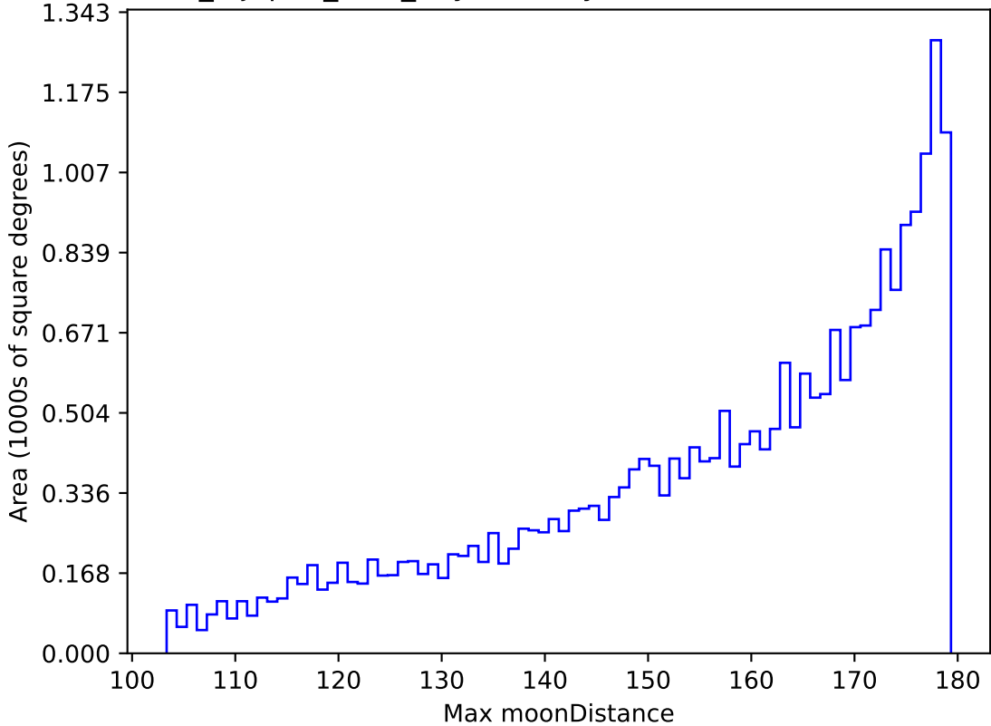
noroll_mjdp60_v3.4_10yrs All sky r band: Max moonDistance
