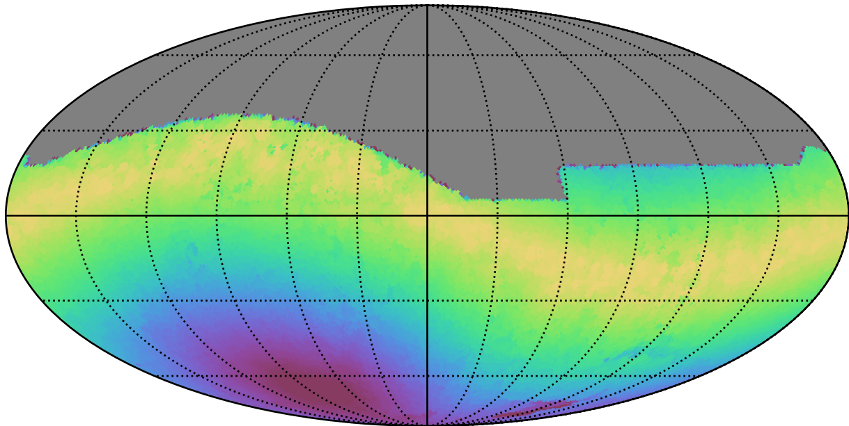
noroll_mjdp60_v3.4_10yrs All sky i band: Max moonDistance
