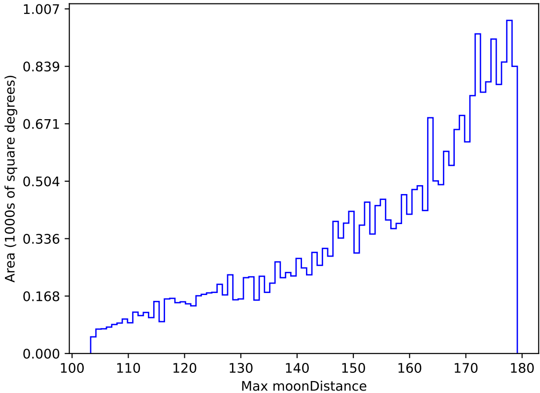
noroll_mjdp60_v3.4_10yrs All sky i band: Max moonDistance
