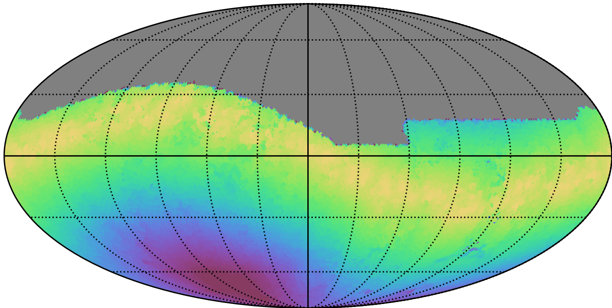
noroll_mjdp60_v3.4_10yrs All sky g band: Max moonDistance
