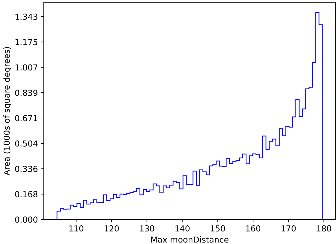
noroll_mjdp60_v3.4_10yrs All sky all bands: Max moonDistance
