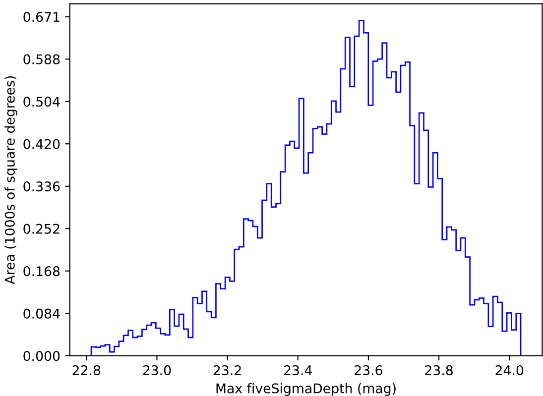
noroll_mjdp60_v3.4_10yrs Yr 1 u band: Max fiveSigmaDepth
