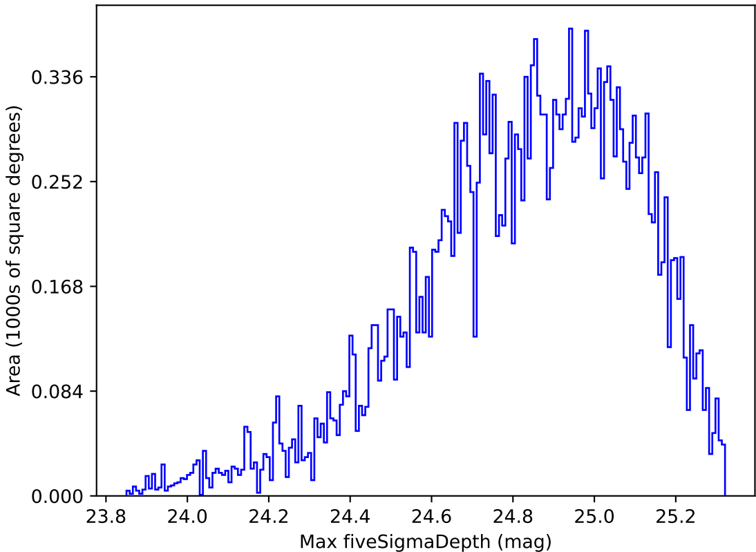
noroll_mjdp60_v3.4_10yrs Yr 1 all bands: Max fiveSigmaDepth
