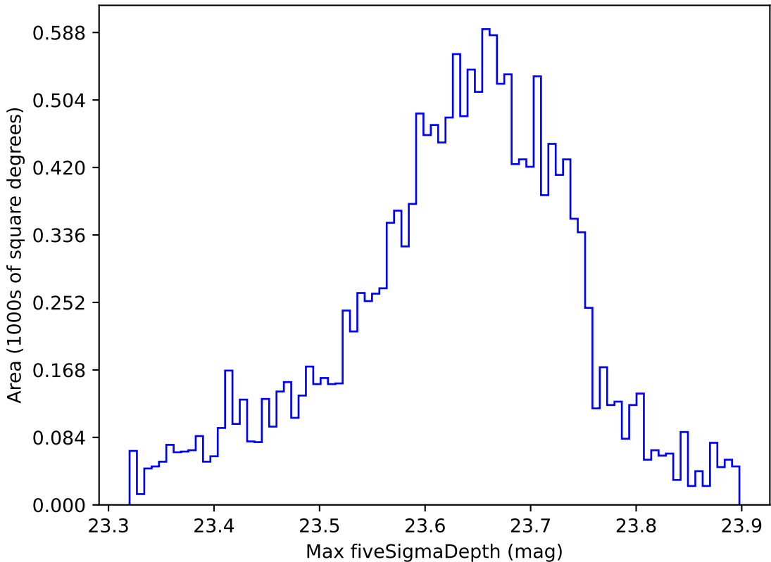
noroll_mjdp60_v3.4_10yrs WFD z band: Max fiveSigmaDepth
