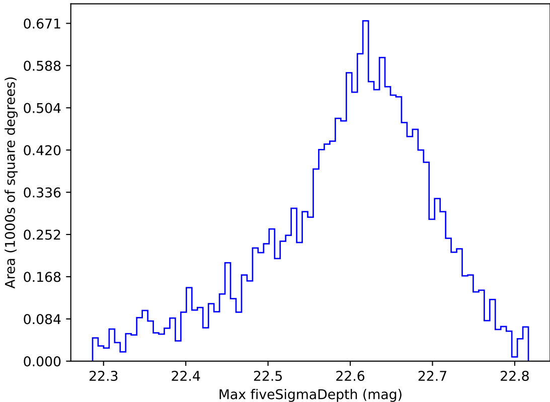
noroll_mjdp60_v3.4_10yrs WFD y band: Max fiveSigmaDepth
